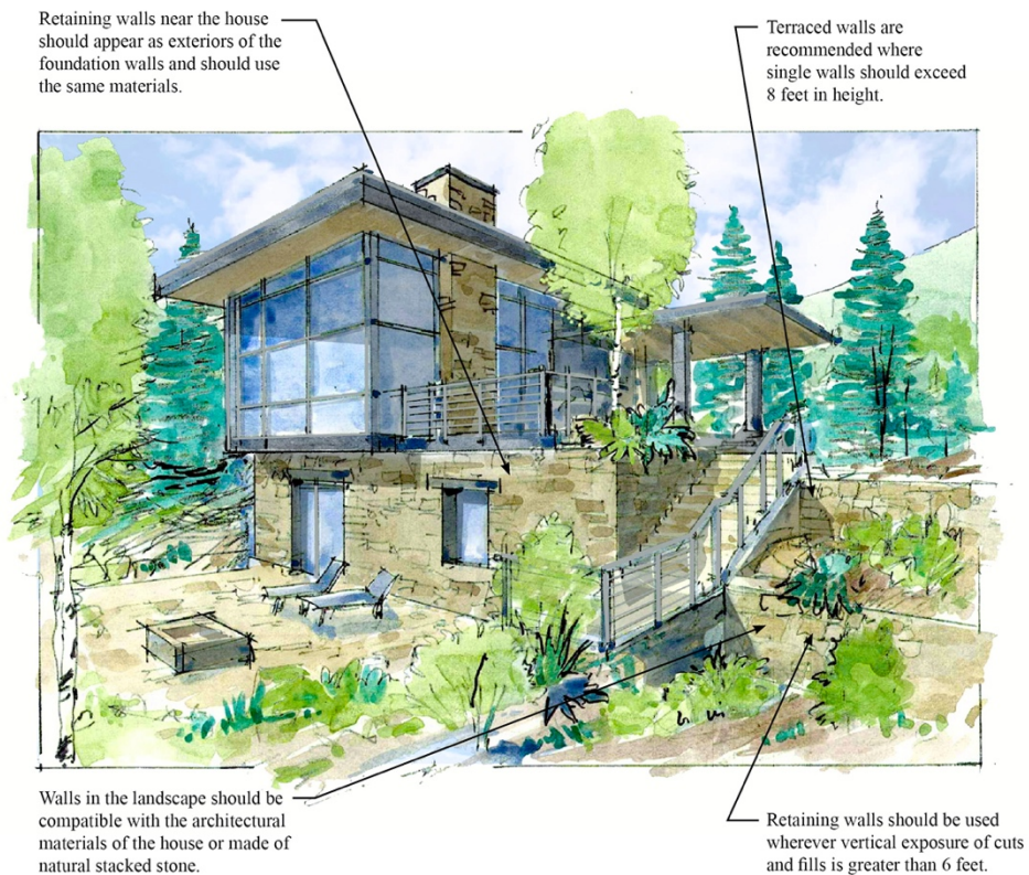
Figure 12: Retaining Walls
